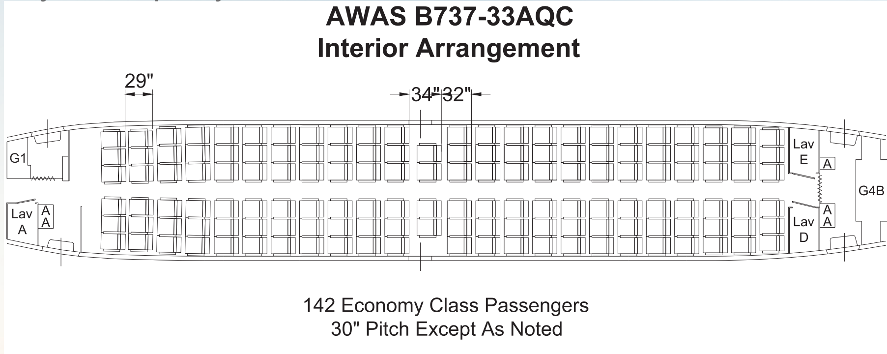
FIGURE 1: Passenger Configuration
